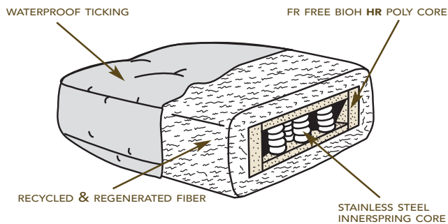
OUTDOOR SPRING FIBER CUSHION
